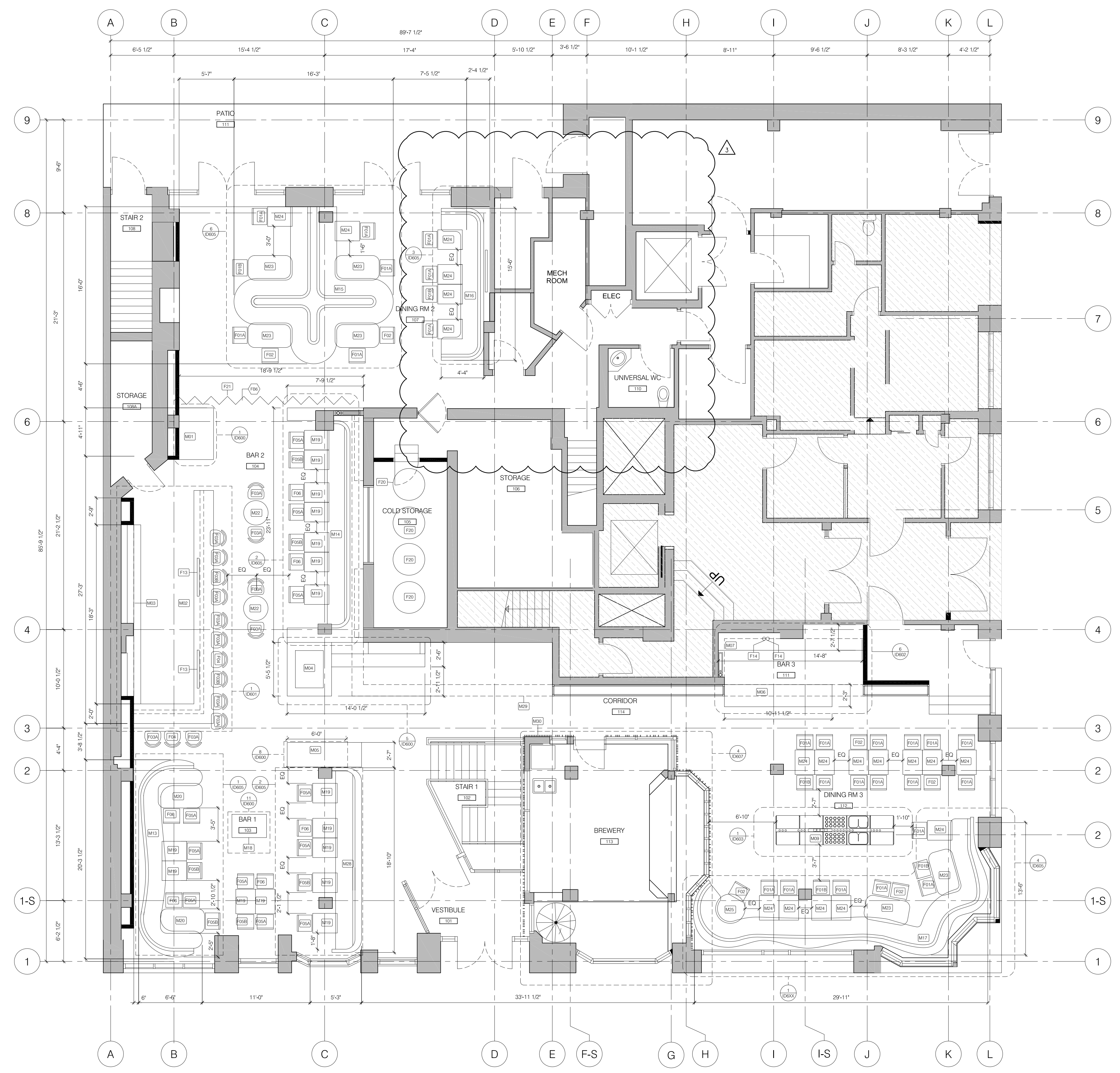
1 GROUND FURNITURE PLAN ID105 Scale: 3/16"=1'-0"
