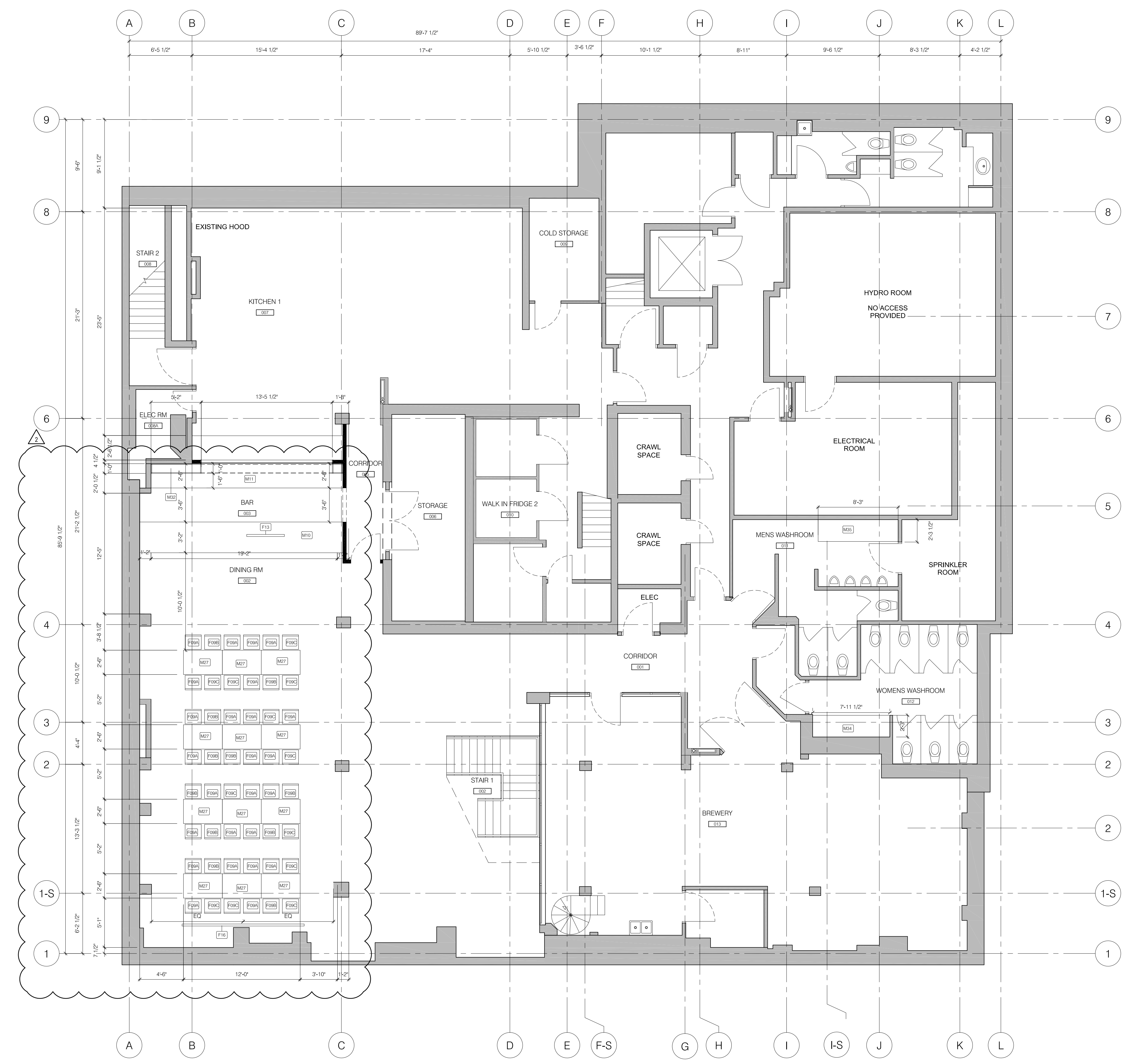
1 BASEMENT FURNITURE PLAN Scale 3/16"=1'-0"
